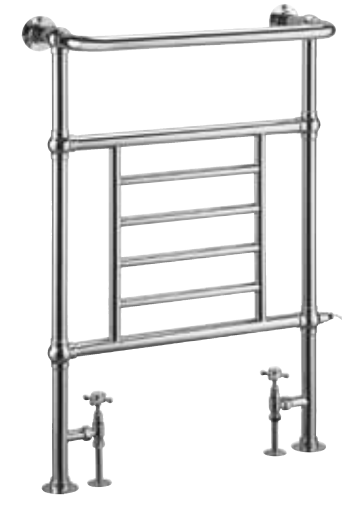
Vincent 600 x 950h x 231mm Chrome £589.00 206w Δ T50
