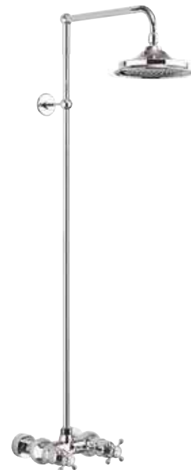
Eden Exposed (Fixed Head) Exposed thermostatic shower valve with rigid riser, 6" fixed head. White £704.00 Black £728.00 Dual control: 1 control for temperature and 1 control for water flow
