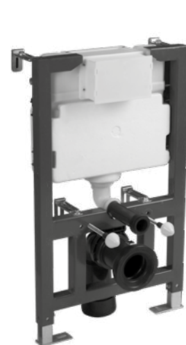
0.82m Wall Hung WC Frame 500(w) x 820(h) x 167-215(d)mm
