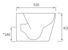
RIMLESS BACK TO WALL PAN
