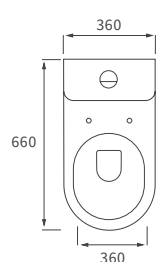
RIMLESS CLOSE COUPLED PAN AND CISTERN
