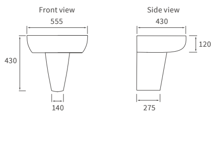
BASIN WITH SEMI PEDESTAL
