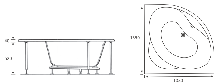
LAGUNA CORNER BATH
