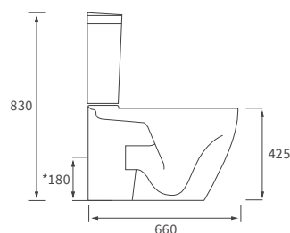
RIMLESS CLOSE COUPLED PAN AND CISTERN
