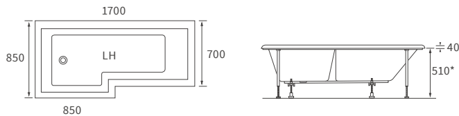
SOLARNA 1700 L SHAPE SHOWER BATH LH AND RH
