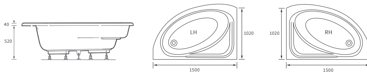
ORLANDO CORNER BATH LH AND RH
