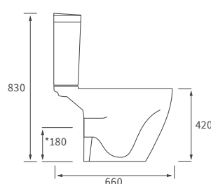
RIMLESS CLOSE COUPLED PAN AND CISTERN
