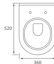
RIMLESS WALL HUNG PAN
