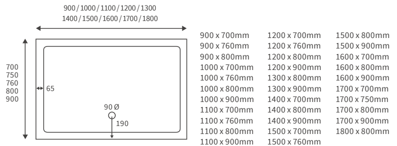
LOW PROFILE RECTANGULAR TRAYS
