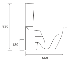
CLOSE COUPLED PAN AND CISTERN
